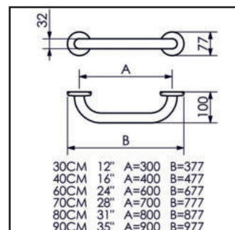
30/40/60/70/80/90 BARRA DE APOIO RETA
